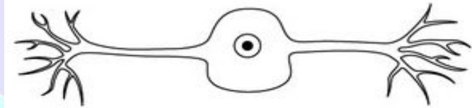
Bipolar neuron
